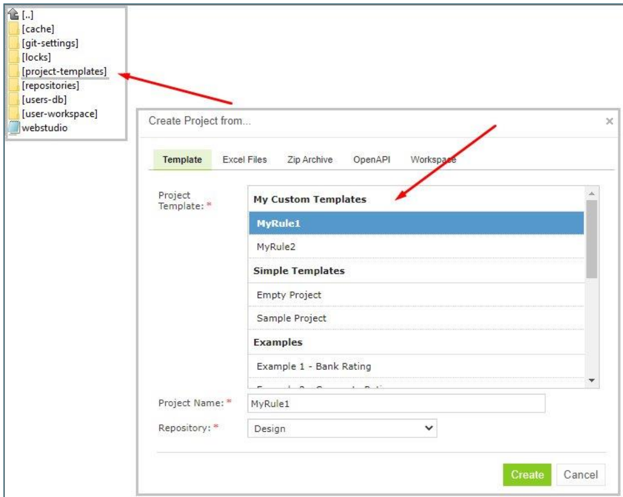
Figure 122: Creating a custom project template
