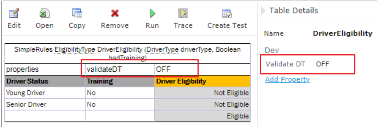
Figure 92: Properties for the Decision table type
