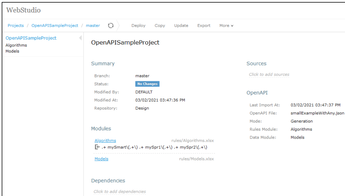
Figure 75: OpenAPI project in Rules Editor, in the Generation mode.
