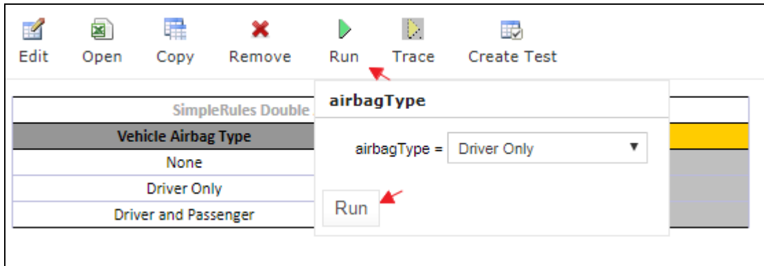
Figure 105: Testing a rule table without tests
