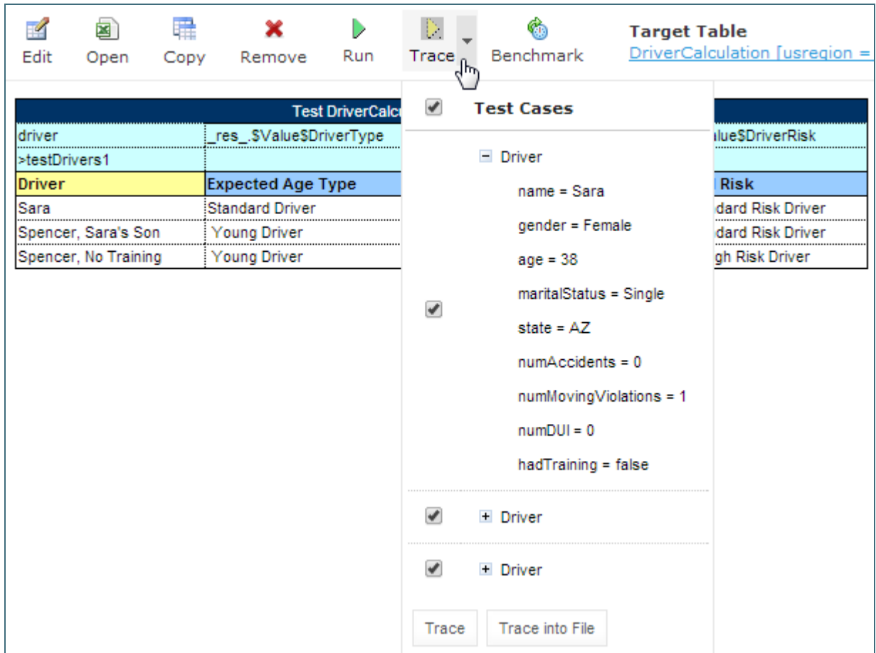
Figure 116: Tracing of a Test table
