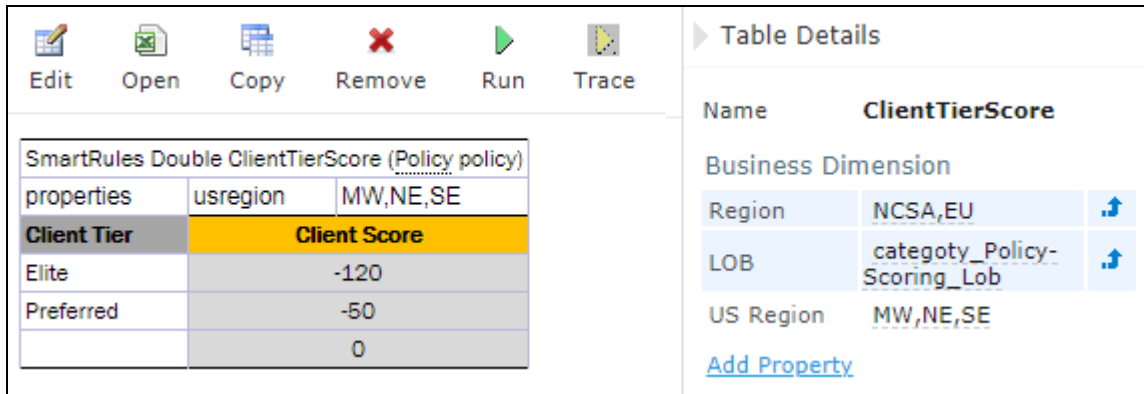
Figure 88: An example of inherited category-level properties
