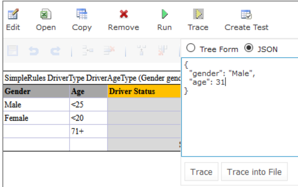
Figure 115: Selecting the JSON option for tracing
