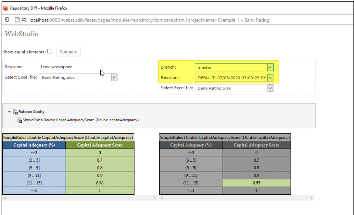
Figure 145: Comparing the current project revision from user workspace to the second project revision
