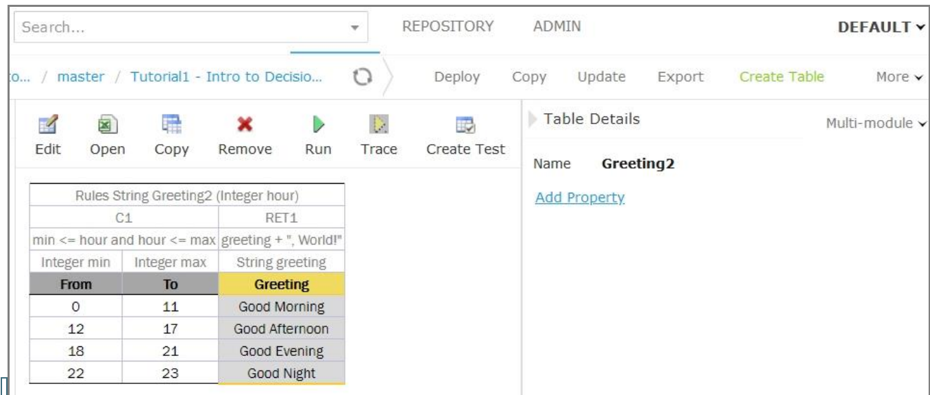
Figure 6: OpenL Tablets WebStudio Rules Editor
