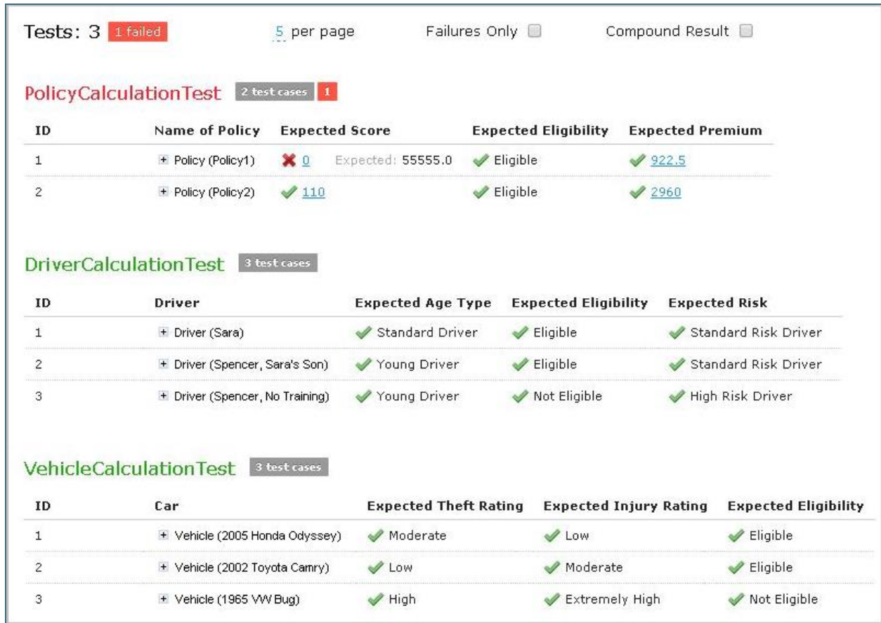
Figure 102: Results of running all project tests
