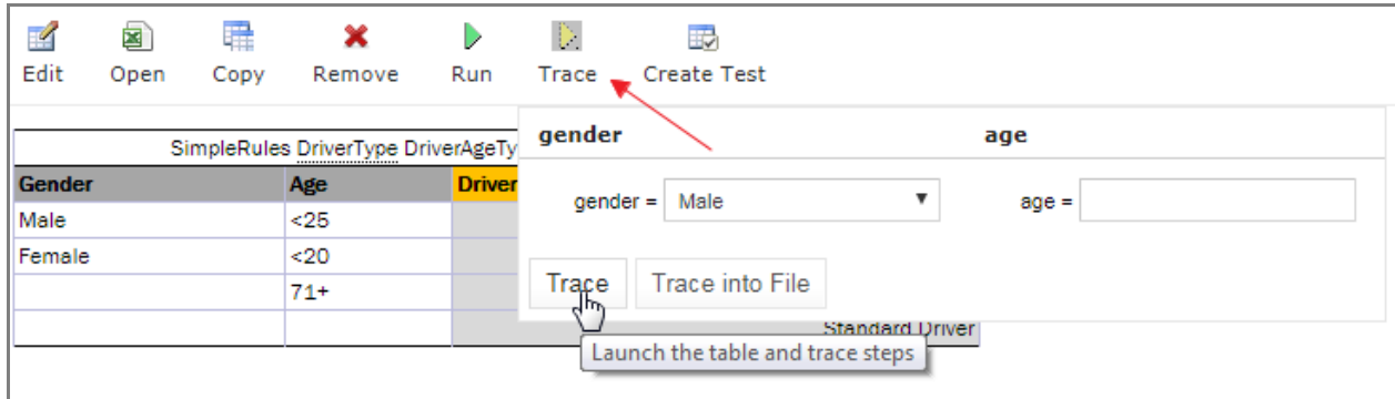
Figure 114: Tracing a rule for a rule table
