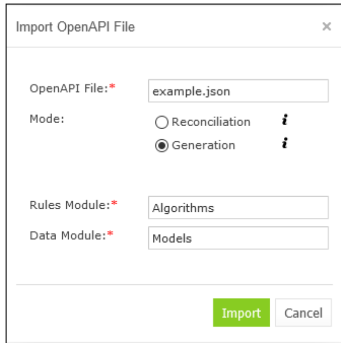
Figure 78: Selecting the generation mode
