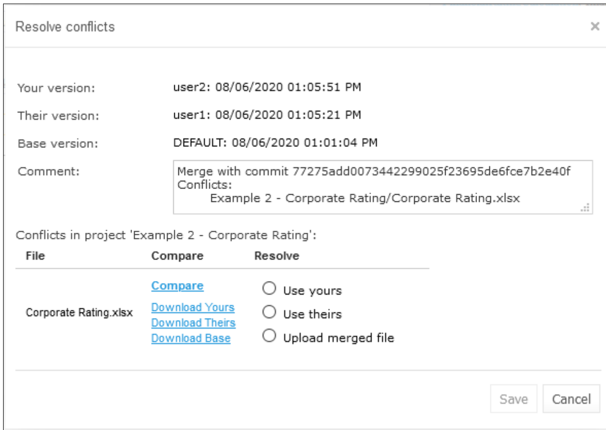
Figure 151: Resolving conflicts on merging branches
