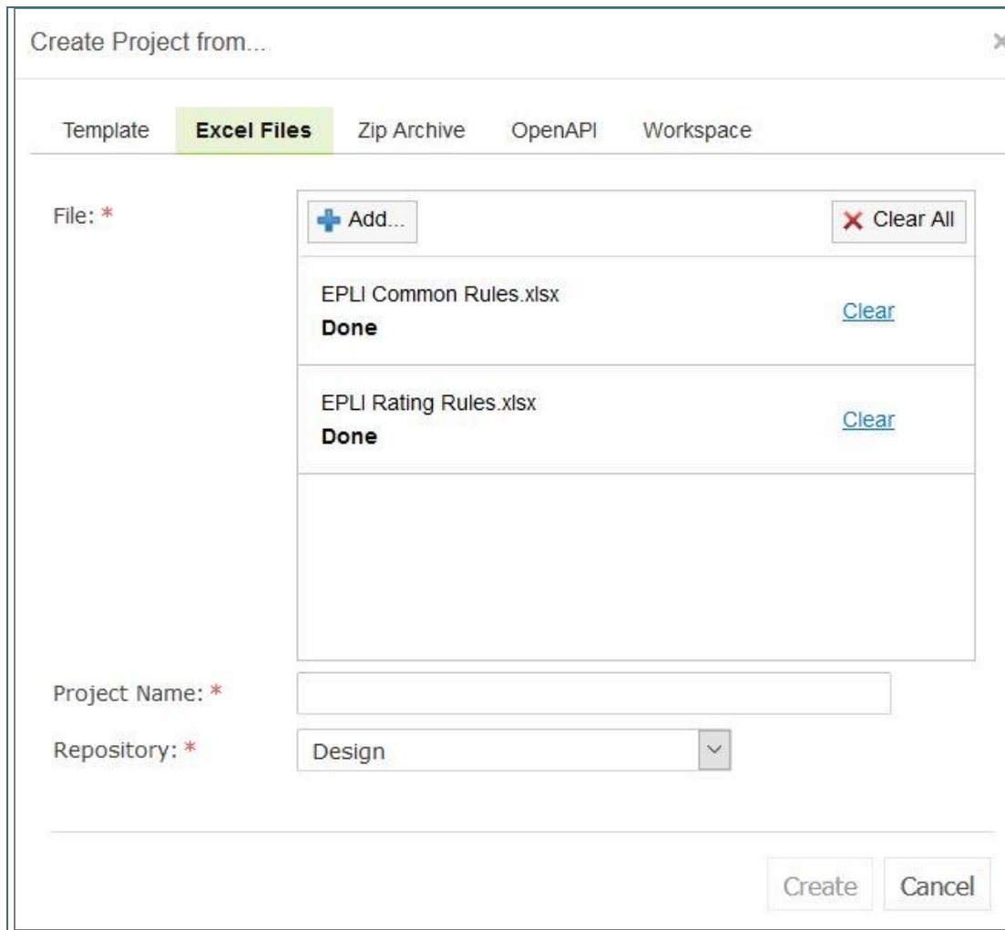
Figure 123: Creating a project from Excel files
